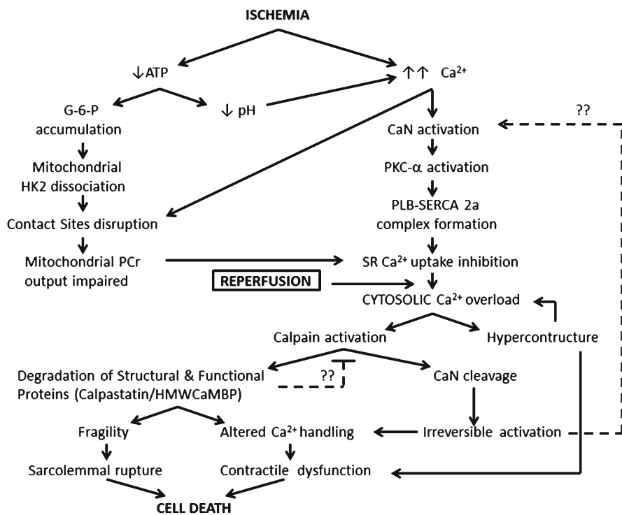
Fig. 1 Schematic representation of calpain-Ca 2+ signaling in myocardial ischemia. The dotted lines with query symbols represent hypothesised pathways. G-6-P indicates Glucose-6-Phosphate; HK—Hexokinase; PCr—phosphocreatine; HMWCaMBP—High Molecular Weight Calmodulin-Binding Protein; CaN—Calcineurin; PKC- \alpha —Protein Kinase C- \alpha ; PLB—Phospholamban; SERCA—Sarcoendoplasmic Reticulum Calcium Transport ATPase
