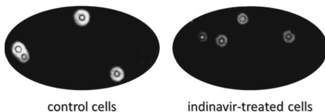
Fig. 12 Effect of indinavir on capsule size of C. neoformans . The yeast cells were cultured in the absence or in the presence of 10 \mu M indinavir for 72 h. In order to evaluate capsule synthesis, C. neoformans was stained with India ink. The images of the most-representative capsule size-related events observed in untreated cells (very large capsules) and indinavir-treated cells (reduced capsules)
