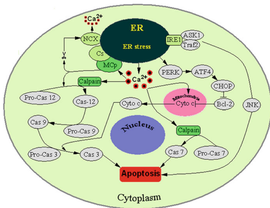
Fig. 2 Mechanisms of induction of apoptosis by ER stress. The direct activation of caspases-12 by \text{Ca}^{2+} dependent calpain activates the caspase-9/caspase-3 cascade. Overload of mitochondria of \text{Ca}^{2+} from the ER leads to the release of proapoptotic factors, such as Cyt C, from mitochondria. Activation of CHOP (C/EBP homologous protein) by PERK/eIF2 \alpha /ATF4 (protein kinase RNA-like ER kinase/eukaryotic initiation factor-2/activating transcription factor 4) leads to the upregulation of pro-apoptotic and down regulation of antiapoptotic Bcl-2 family members IRE1/Traf2/ASK2 (inositol requiring protein-1/tumour necrosis factor receptor-associated factor 2/ASK2) activates JNK (c-Jun N-terminal Kinase) signaling to trigger apoptotic pathways ER stress-mediated increased \text{Ca}^{2+} may also activate the ER associated MCp, which then activates the pro-caspase 12 and induces caspase 12 mediated apoptosis and this activated MCp may also cleave the ER \text{Ca}^{2+} uptake protein NCX, which is the main cause of secondary \text{Ca}^{2+} overload in the cytosol and cellular dysfunction
