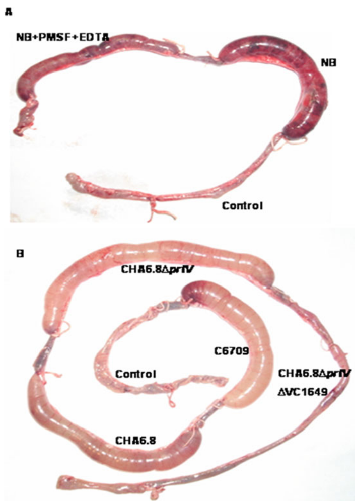
Fig. 5 Rabbit ileal loop assay. (a) RIL response of partially purified protease (50 \mu g, NB) showing significant hemorrhagic fluid accumulation (FA ratio 1.2 \pm 0.2 n=3 ) and its effect after inhibition with 25 mM PMSF and 10 mM EDTA (NB+PMSF+EDTA) shows significant decrease in fluid accumulation (FA ratio 0.3 \pm 0.05 n=3 ). Twenty five mM Tris-HCl with 25 mM PMSF+ 10 mM EDTA was used as a negative control (FA ratio= 0.12 \pm 0.002 , n=3 ). (b) RIL response with culture supernatants of C6709 (FA ratio 1.1 \pm 0.3 , n=3 ), CHA6.8 (FA ratio 1.08 \pm 0.2 , n=3 ), CHA6.8 \Delta prtV (FA ratio 1.02 \pm 0.2 , n=3 ), CHA6.8 \Delta prtV \Delta VC1649 (FA ratio 0.11 \pm 0.005 , n=3 ) and Tryptic soy broth as negative control (FA ratio 0.09 \pm 0.002 , n=3 )
