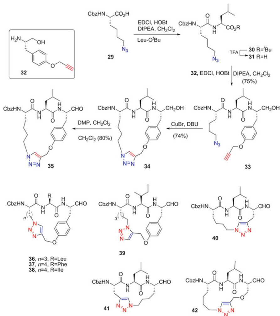
Fig. 8 Macrocyclic inhibitors prepared by azide-alkyne cycloaddition
