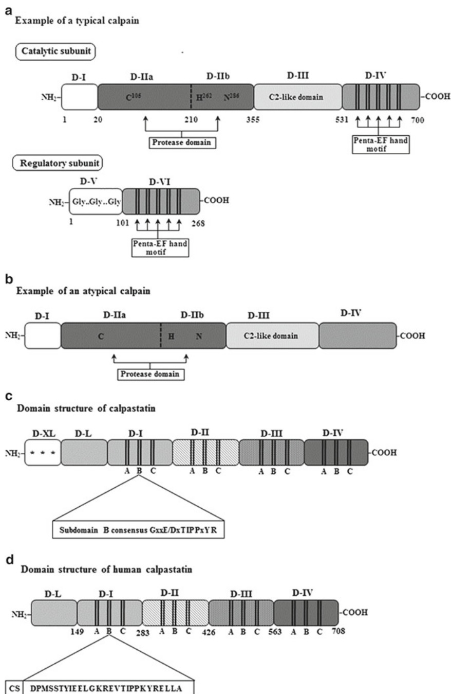
Fig. 1 Schematic diagram of calpains and calpastatin molecules. (a) Schematic representation of domain architecture of the typical calpains. The catalytic subunit contains domains I–IV. Domain I
