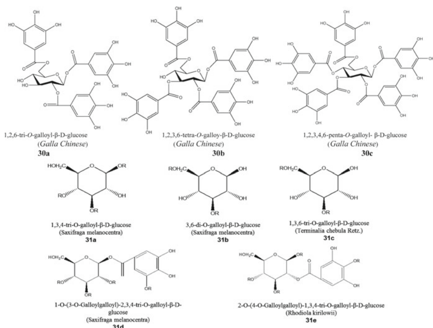
Fig. 18 Structures and resources of polyphenols from natural sources
